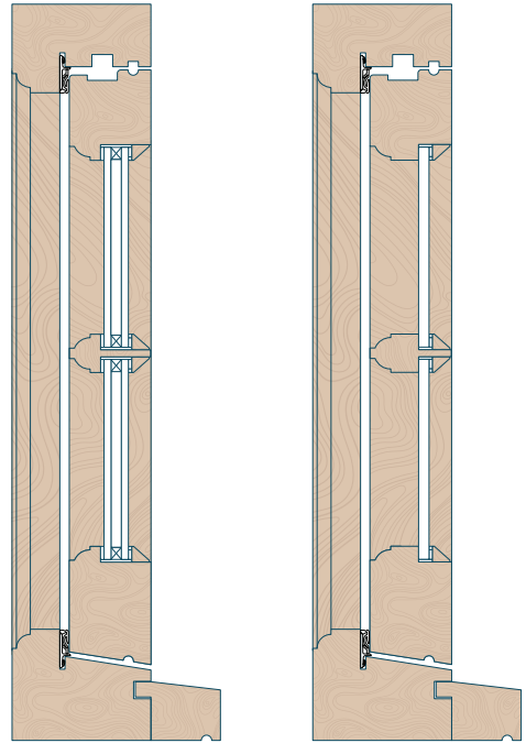
1 Double Glazed (16mm)
