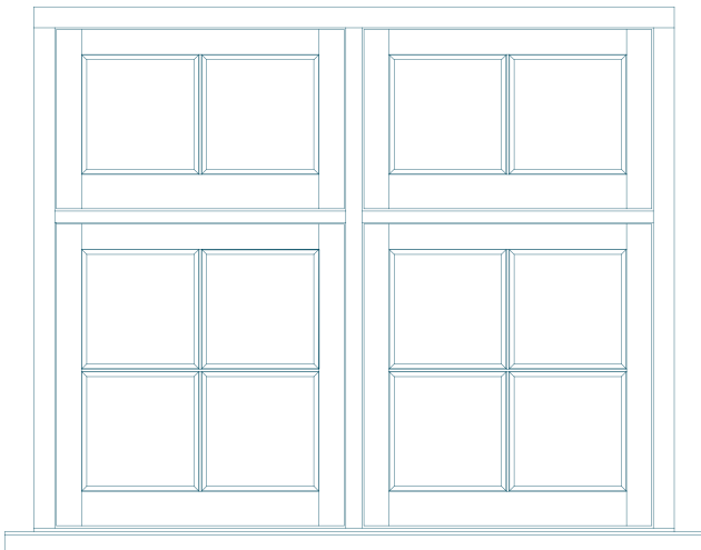
Twin Casement with Fan Lights and Mullion
